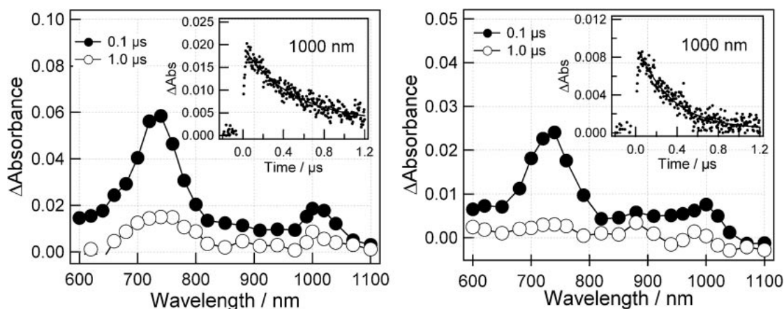
Fig. 6. Transient absorption spectra of C_{60} -TPA- C_{60} obtained by 532 nm laser light in Ar-saturated BN (left) and DMF (right).
