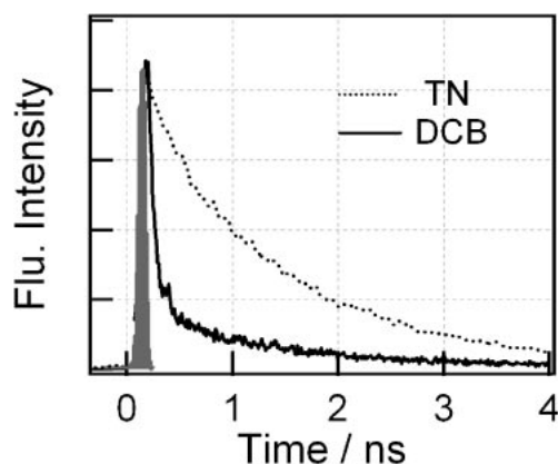
Fig. 3. Time profiles of ^1C_{60}^* -fluorescence at 710 nm of C_{60} -TPA- C_{60} 1 in toluene (TN) and DCB; \lambda_{\text{ex}} = 400 nm.
