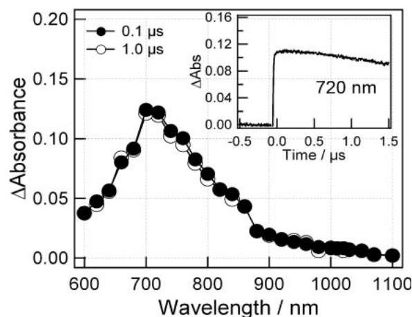
Fig. 5. Transient absorption spectra of C 60 -TPA-C 60 1 obtained by irradiating 532 nm laser light in Ar-saturated toluene.
