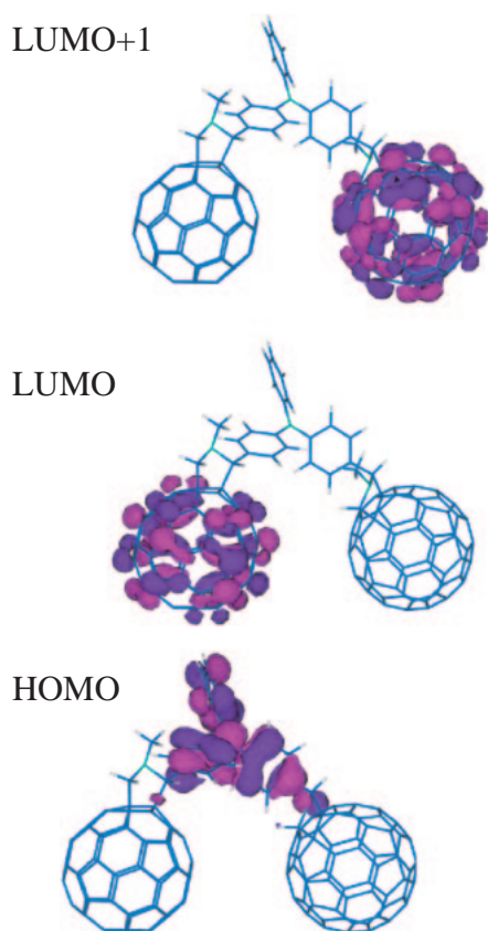
Fig. 4. Optimized structure and the HOMO, LUMO, and LUMO+1 of C 60 -TPA-C 60 calculated by ab initio molecular orbital method at B3LYP/3-21G level.
