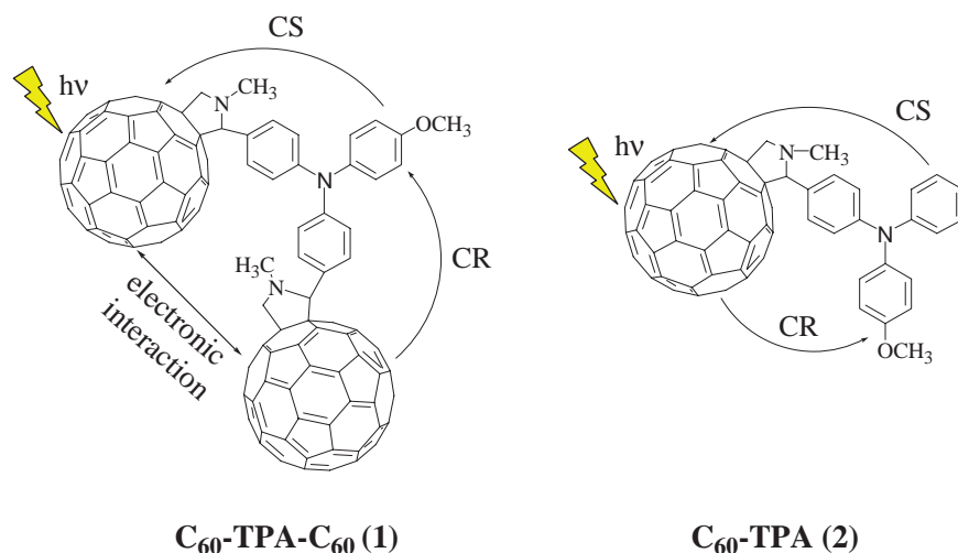
Fig. 1. Molecular structures and expected photoinduced processes: CS; charge separation, CR; charge recombination. In the present study, TPA refers as to CH 3 O-substituted triphenylamine otherwise cited.
