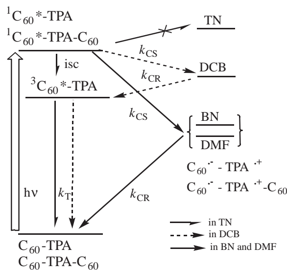
Fig. 7. Energy diagram of C_{60} -TPA- C_{60} and C_{60} -TPA in the studied solvents.
