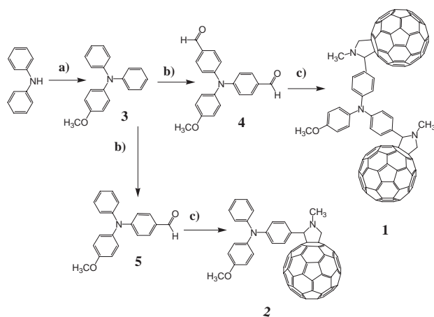
Scheme 1. Synthesis of compounds 1 and 2 ; a) 4-iodoanisole, K 2 CO 3 , Cu, 18-crown-6, o -dichlorobenzene (DCB), 180, 48 h, 86.0% yield, b) POCl 3 , DMF, o -dichloroethane, reflux, 36.7% yield for 4 and 73.0% yield for 5 , and c) sarcosine, fullerene, reflux, 10.0% yield for 1 , 29.0% yield for 2 .
