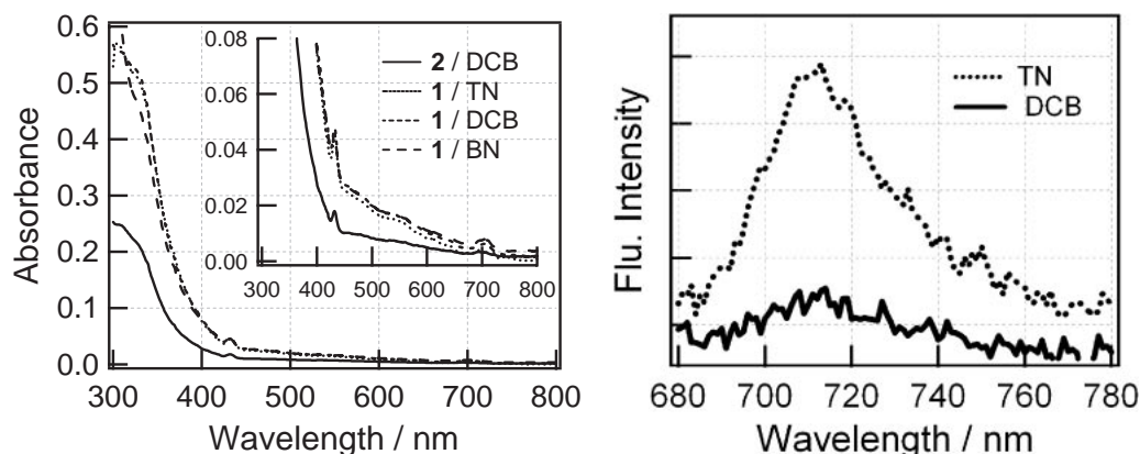
Fig. 2. Steady-state absorption of C_{60} -TPA- C_{60} 1 and C_{60} -TPA 2 (left) and fluorescence spectra (right) of C_{60} -TPA- C_{60} in toluene (TN), and o -dichlorobenzene (DCB); \lambda_{\text{ex}} = 400 nm. Concentrations are kept at 1 \times 10^{-6} mol dm ^{-3} .
